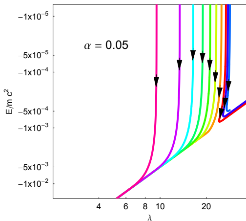
Fig. 2. Angular momentum ( \lambda = \frac{h}{2m\tau_{\text{gc}}} ) - orbital energy ( E ) during the tidal evolution of the orbit for the evolution tracks shown in the right panel of Fig. 1.
