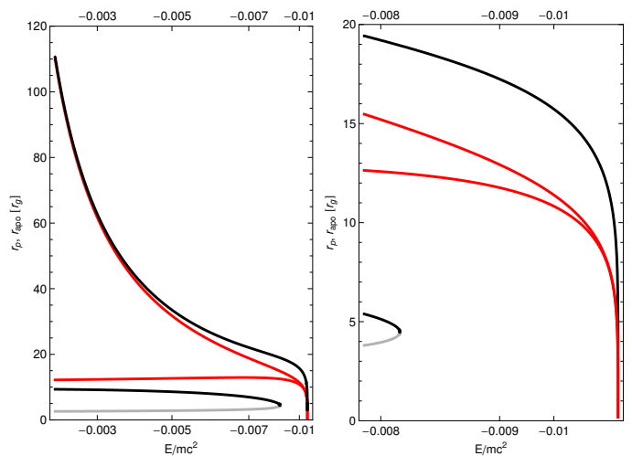
Fig. 3. The evolution of radial turning points in the Kepler (red) and Schwarzschild effective potentials (black) for the case of a highly eccentric orbit starting with periastron at 9.5r_g and apostron at 110r_g . The right figure is an enlargement of the final evolution. The gray line indicates the third root of the effective potential equation (Misner, Thorne & Wheeler 1971).
